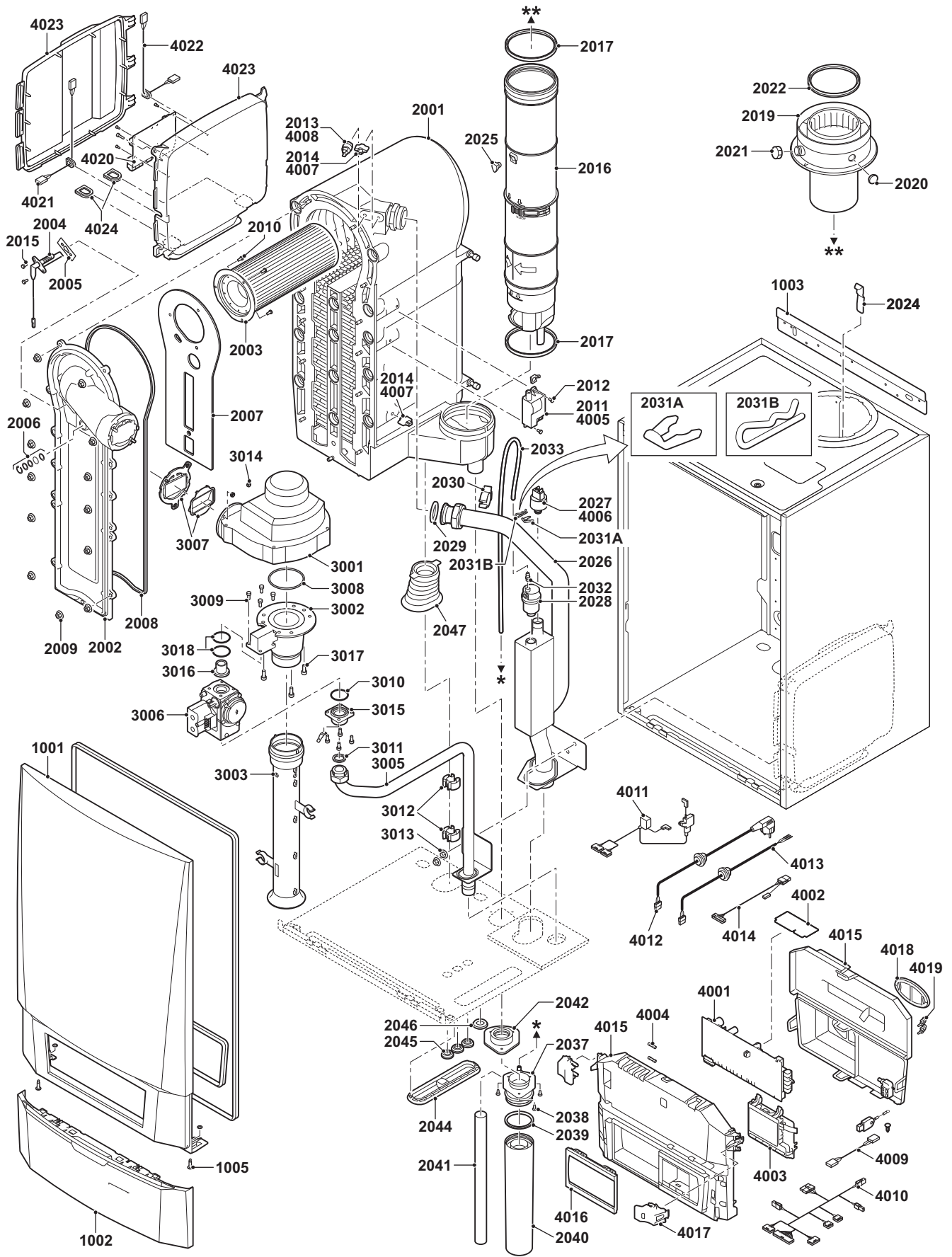
Fig.69 Quinta Pro 115
