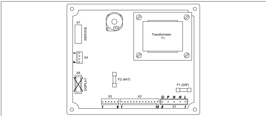
fig. 14 Circuit imprimé Gasmodul
