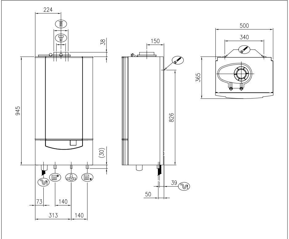
fig. 04 Dimensions Remeha Quinta 25s et Quinta 30s
