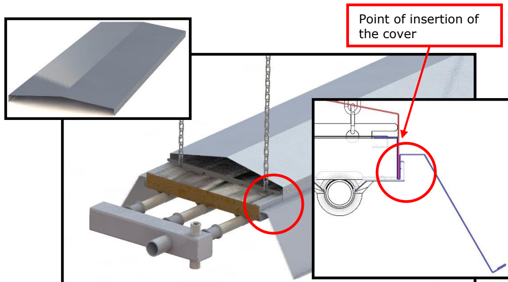
Fig. 3.31 Covers for panels of 300, 600 and 900 mm width, with anti-convective aprons.
