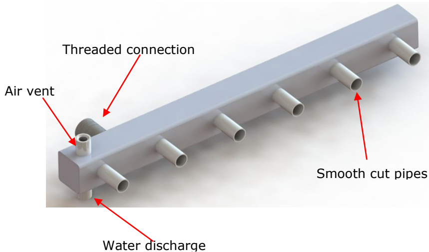
Fig. 1-9 Components of the header
