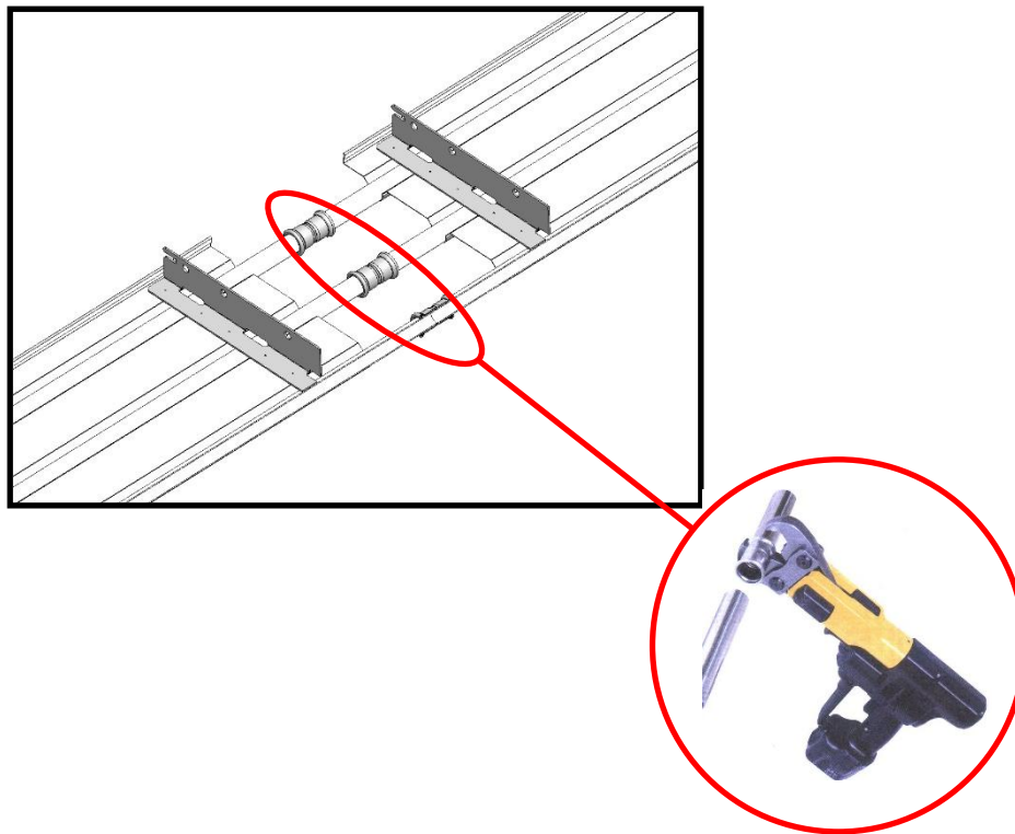
Fig. 3.13c Pinch the sleeve with the suitable tool
