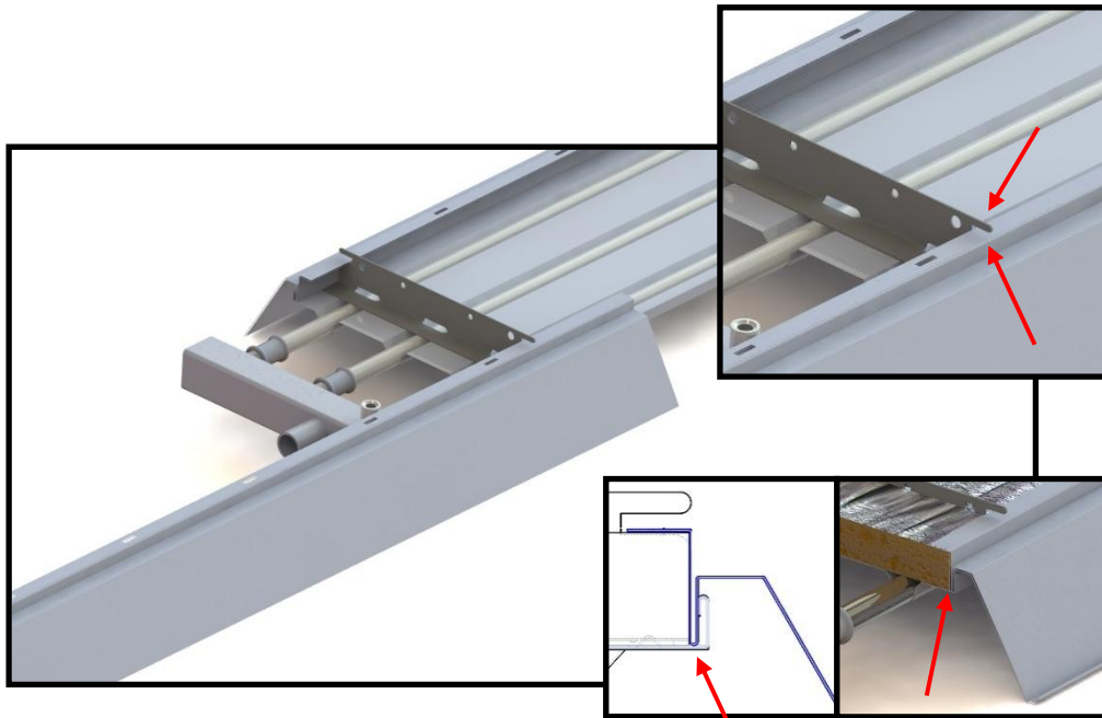
Fig. 3.23 Insertion of the anti-convective aprons.
