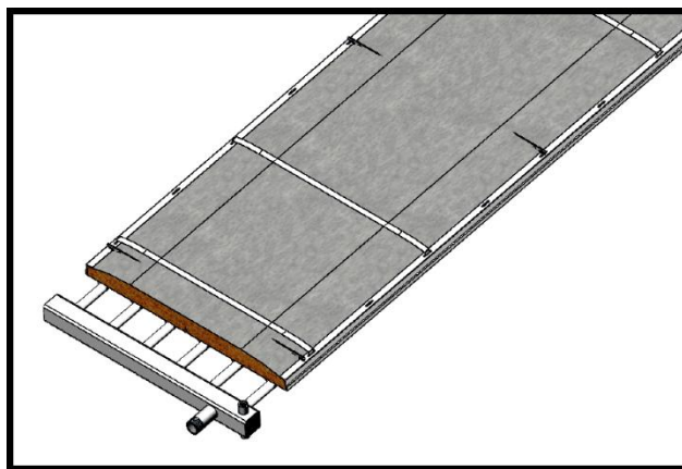
Fig. 3.21 Quantity and positioning of fiberglass holding straps
