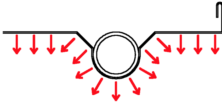
Fig. 1-4 Detail of the radiant sheet
