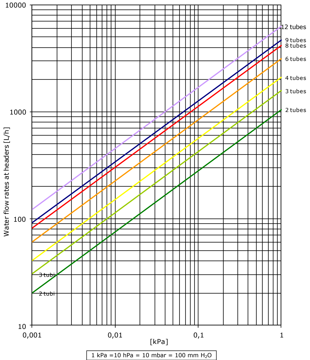
Pressure drop per linear meter of radiant panel with 22.0x1.2 pipe diaphragmed header (average temperature 80 ° C)
