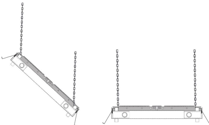
Fig. 3.4 Installation of strip heaters with two anchors
