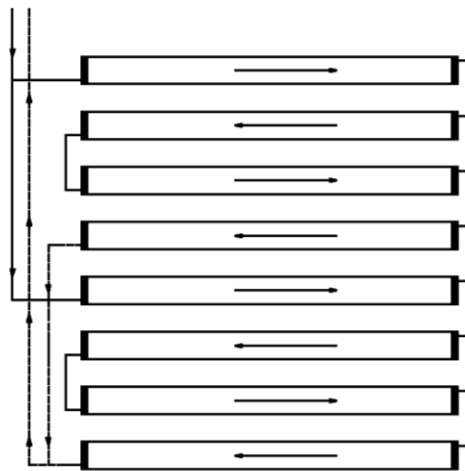
Inlet and outlet on same side - 4 panels in sequence
