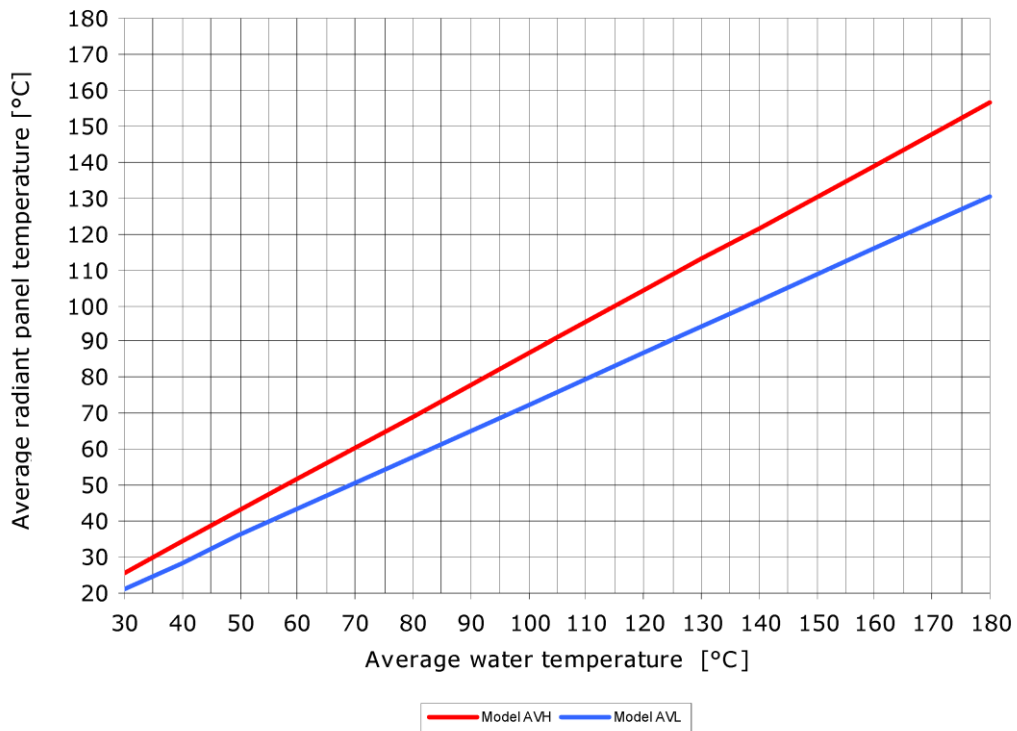
Fig. 1.27 Average surface temperature of the ceiling radiant panel
