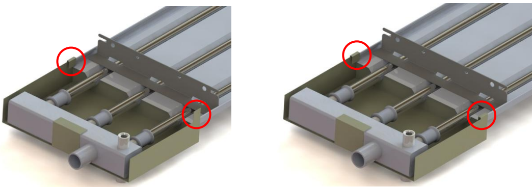
Fig.3.10a Fix the header cover to the panel, bending the special winglet
