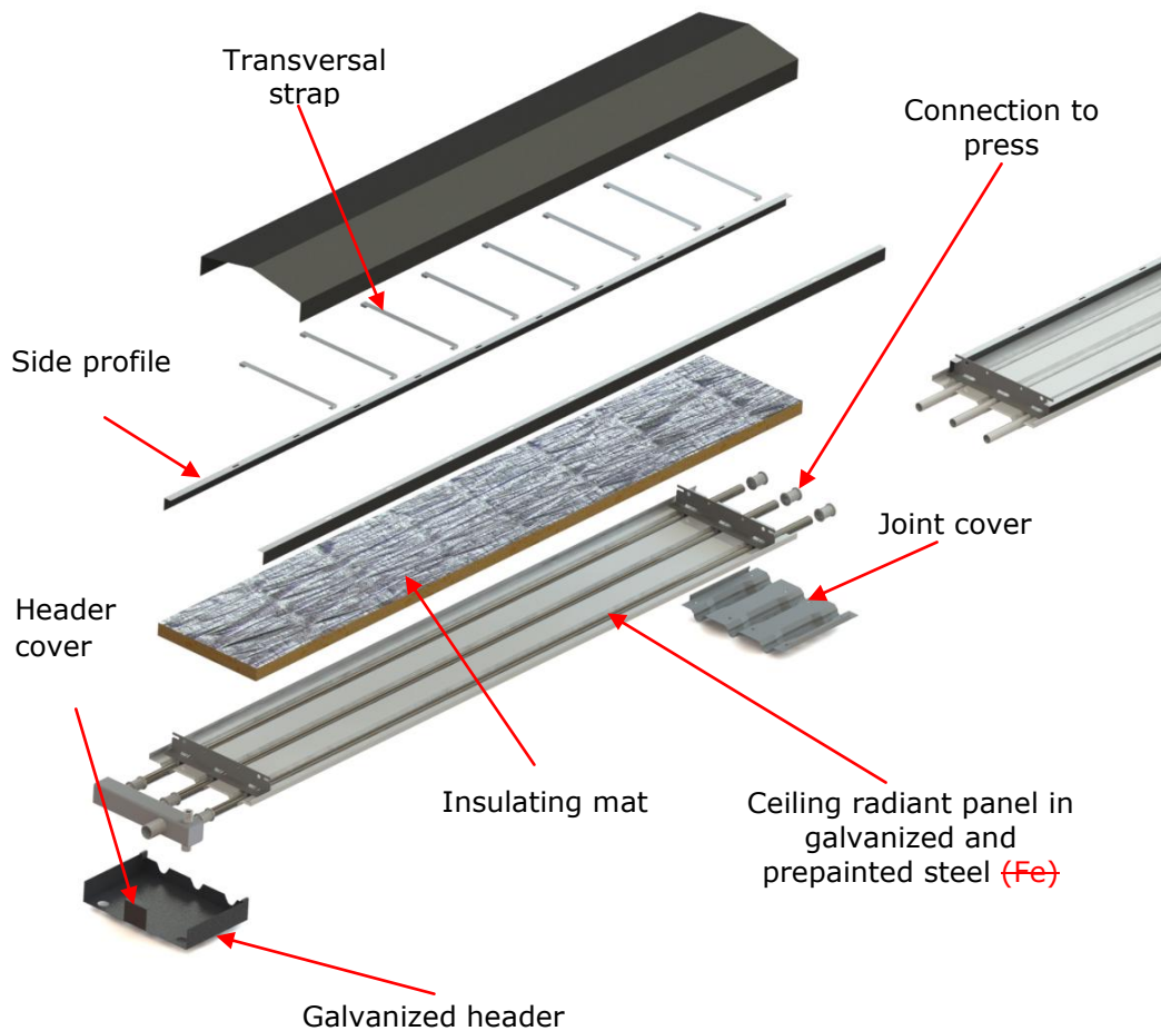
Fig. 1-2 Exploded view of the EUTERM ceiling radiant panel
