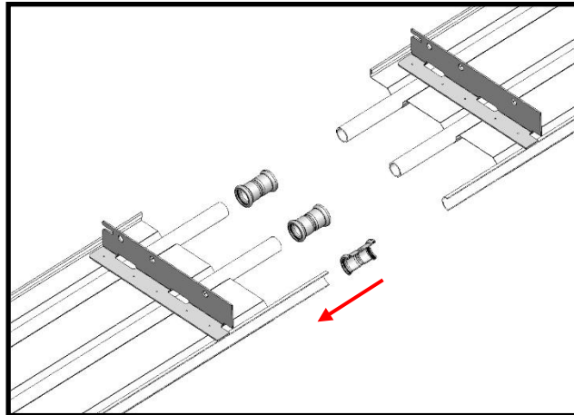
Fig. 3.13 Insert the tubes in the sleeves till reach the bore
