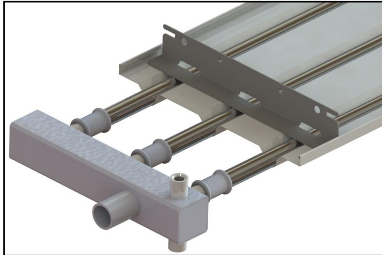
Fig. 3.9e Example of a header connected to the panel
