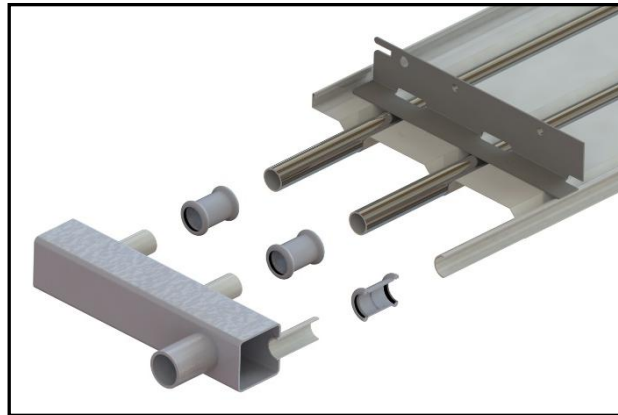
Fig. 3.9 Connection between the header and the pipeline with sleeves to press
