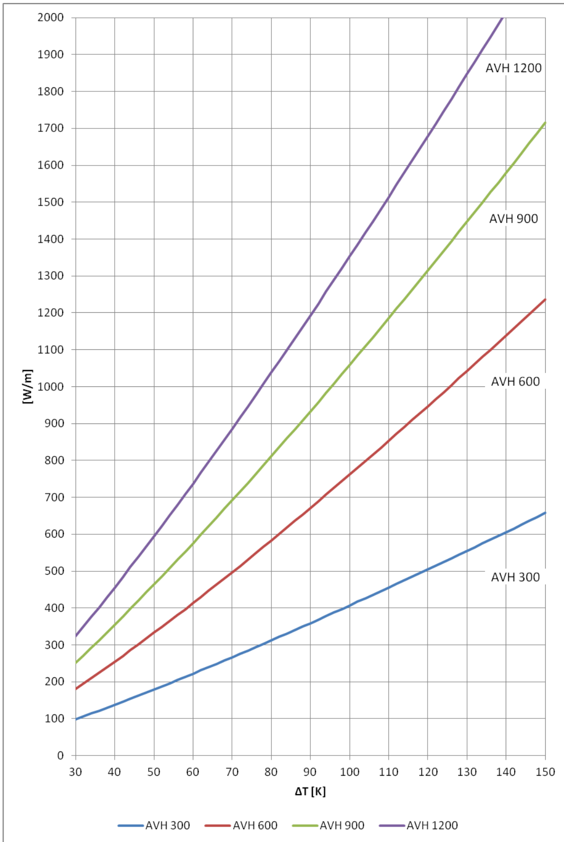
Fig. 1.18 Thermal output for EUTERM AVH in according to EN 14037-1,2,3.
