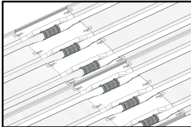
Fig. 3.15 Fastening of joint cover
