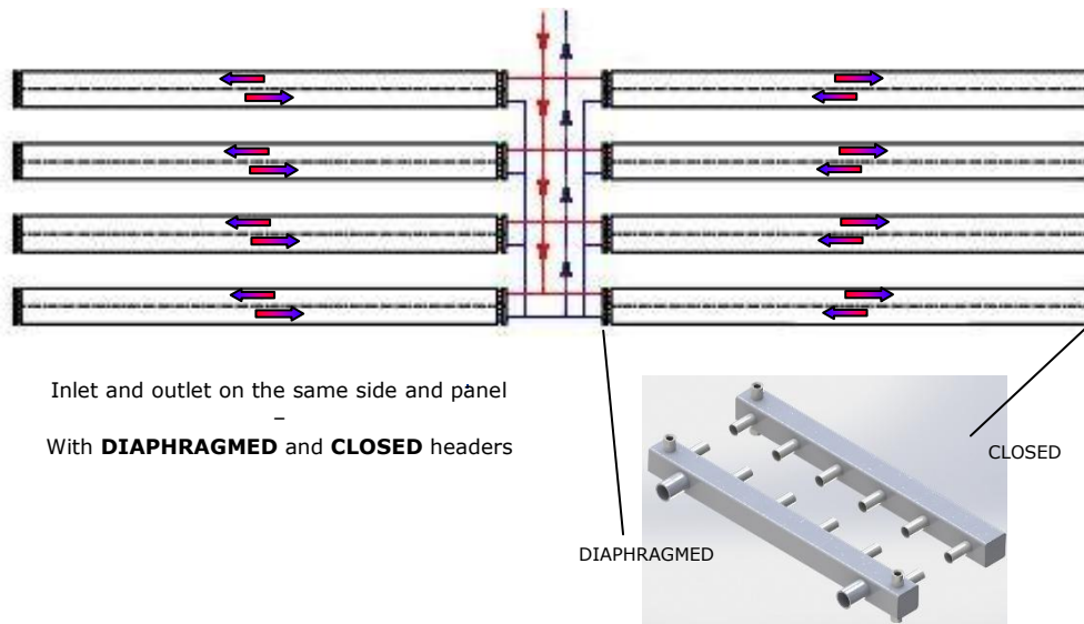
Fig. 3.7 Examples of compensated type circuits with DIAPHRAGMED and CLOSED headers
