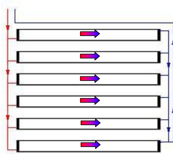
Inlet and outlet on opposite sides - 1 panel Serial fed - With STANDARD headers
