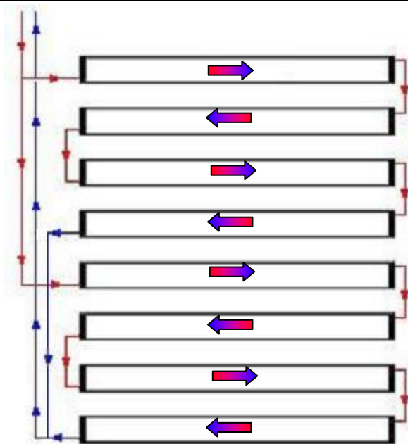
Fig. 3.6 Examples of compensated type circuits with STANDARD headers
