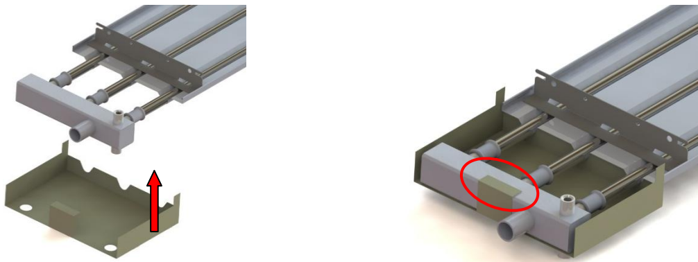
Fig. 3.10 Apply the header cover as shown in the picture below
