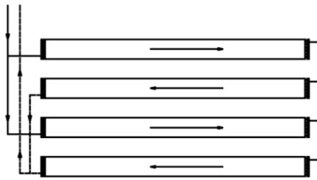
Inlet and outlet on same side - 2 panels in sequence
