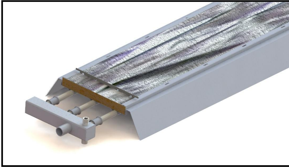
Fig. 3.25 Apply the insulating mat with the paper layer upwards
