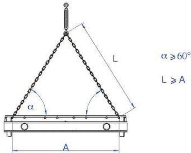
Fig. 3.5 Installation of radiant panel with one anchor
