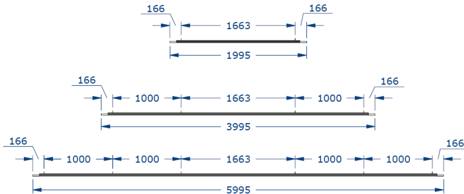
Fig. 3.3 Interval between corner pieces as length of heater strips is varied [mm]
