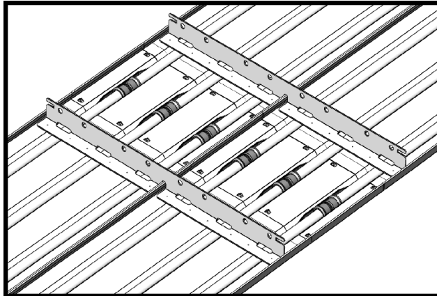
Fig. 3.14 Application of joint cover
