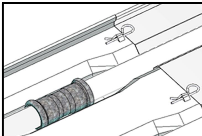
Fig. 3.16 Detail of fastening of joint cover
