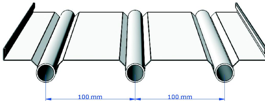
Fig. 1-5 Radiant sheet and tubes
