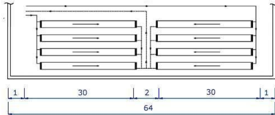
Fig. 2.7 Length of radiant lines
