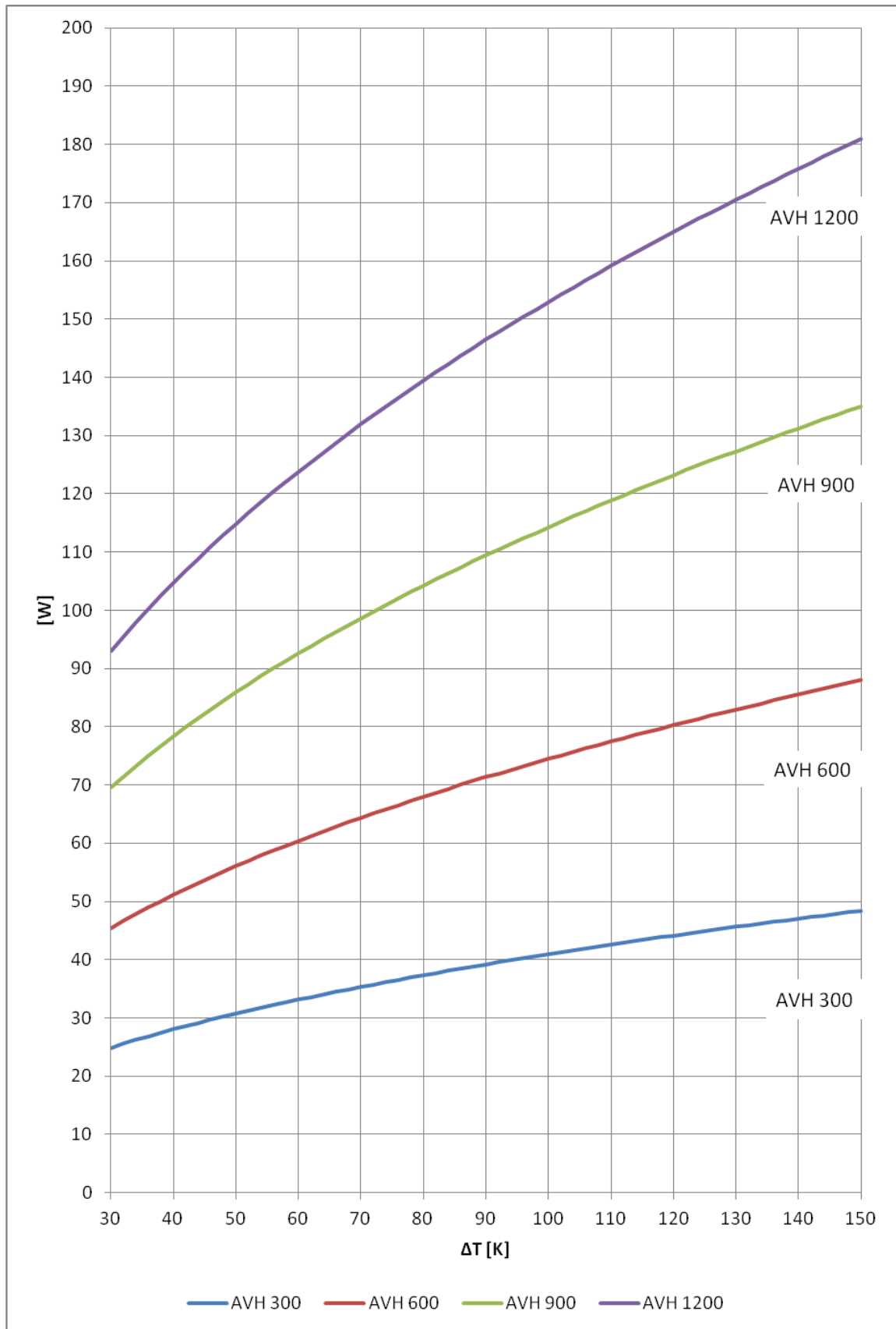
Fig. 1.19 Thermal output for EUTERM AVH headers in according to EN 14037-1,2,3.
