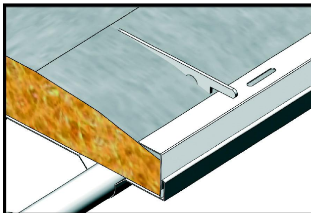
Fig. 3.19 Correct position of the insulating mat after cutting the mat nearby the fixing points and after inserting the mat under the side slats.
