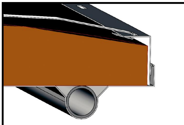
Fig. 3.22 Detail of fastening of fiberglass holding strap
