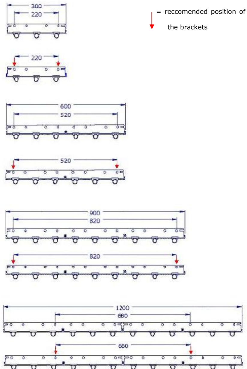
Fig. 3.2 Recommended distance [mm] between brackets when changing width of radiant panel
