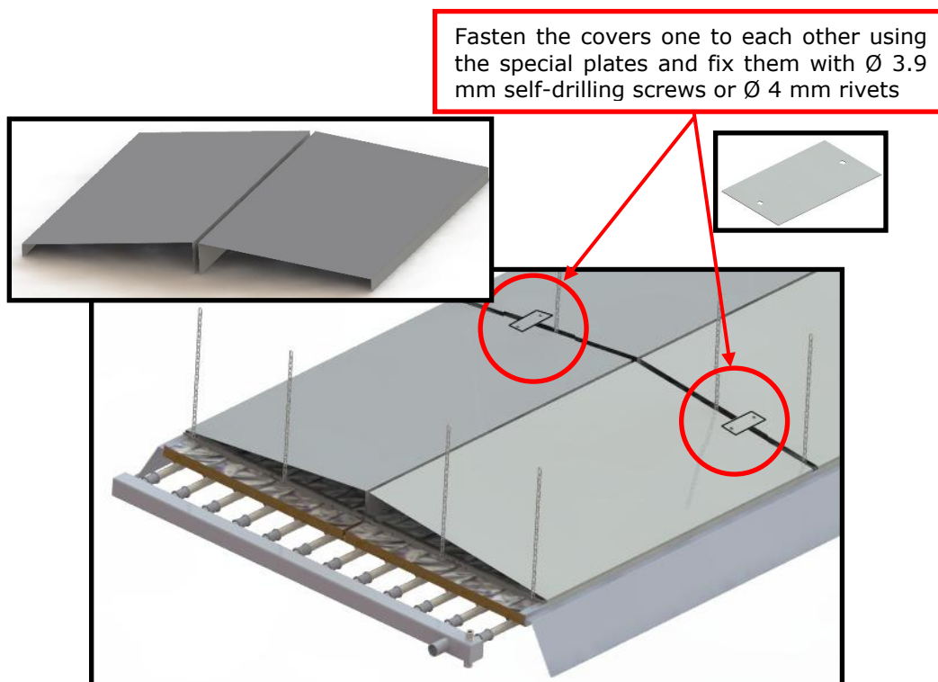
Fig. 3.31 Covers for panels of 300, 600 and 900 mm width, with anti-convective aprons.
