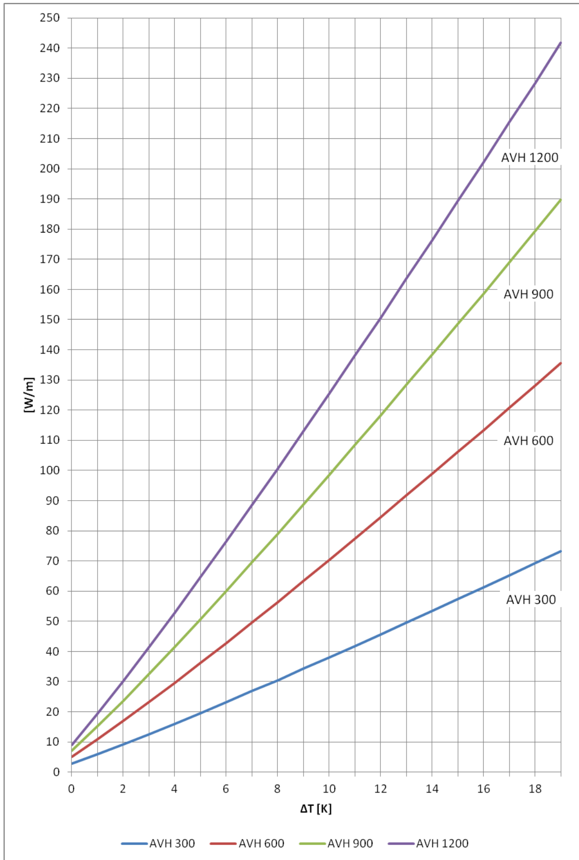
Fig. 1.23 Cooling output for EUTERM AVL ceiling radiant panels
