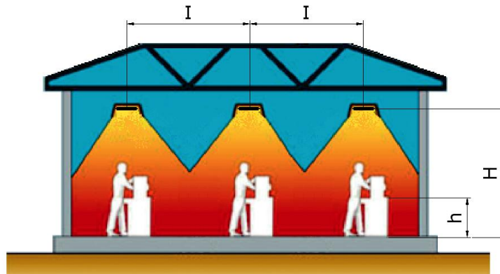
Fig. 2.3 Installation height of the ceiling radiant panels
