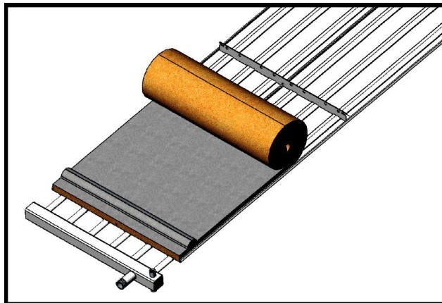
Fig. 3.18 Application of the insulating mat with the paper side up.
