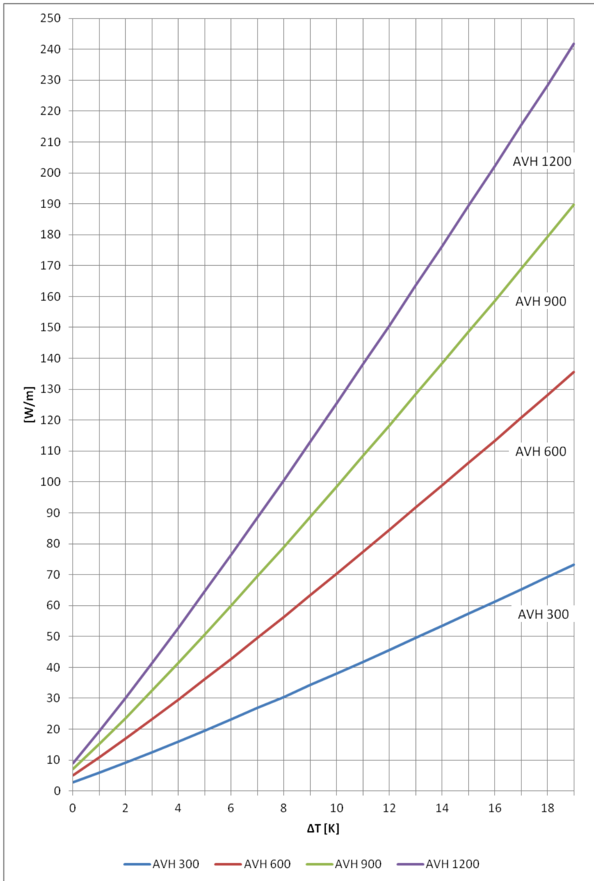
Fig. 1.22 Cooling output for EUTERM AVH ceiling radiant panels in according to EN 14240
