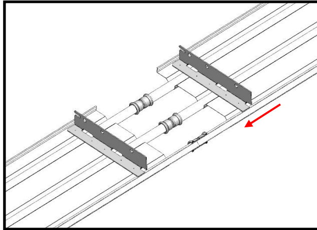
Fig. 3.13b Insert the tubes of the next panels in the sleeves till reach the bore.
