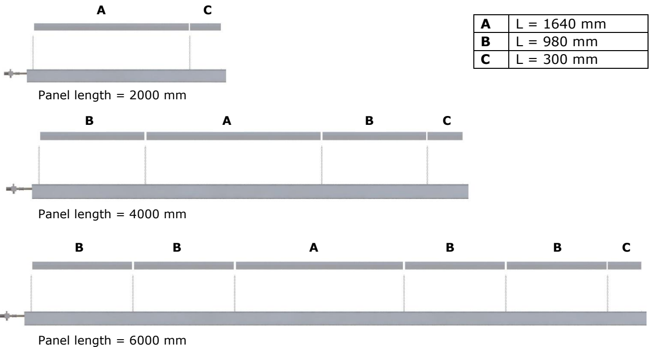
Fig. 3.28 Positioning of the covers
