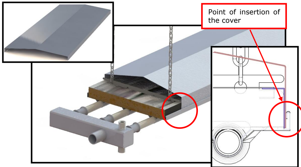
Fig.3.27 Covers for panels of 300, 600 and 900 mm.
