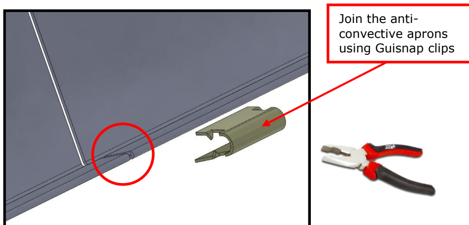
Fig. 3.24 Junction of anti-convective aprons.
