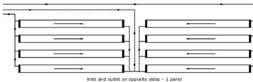
Fig. 2.6 Diagram of the type of circuit selected
