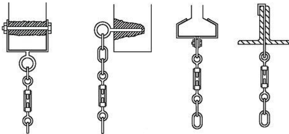
Fig. 3.1 Types of fastening of anchors to the building structure
