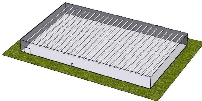
Fig. 2.8 Layout of the radiant lines in the warehouse
