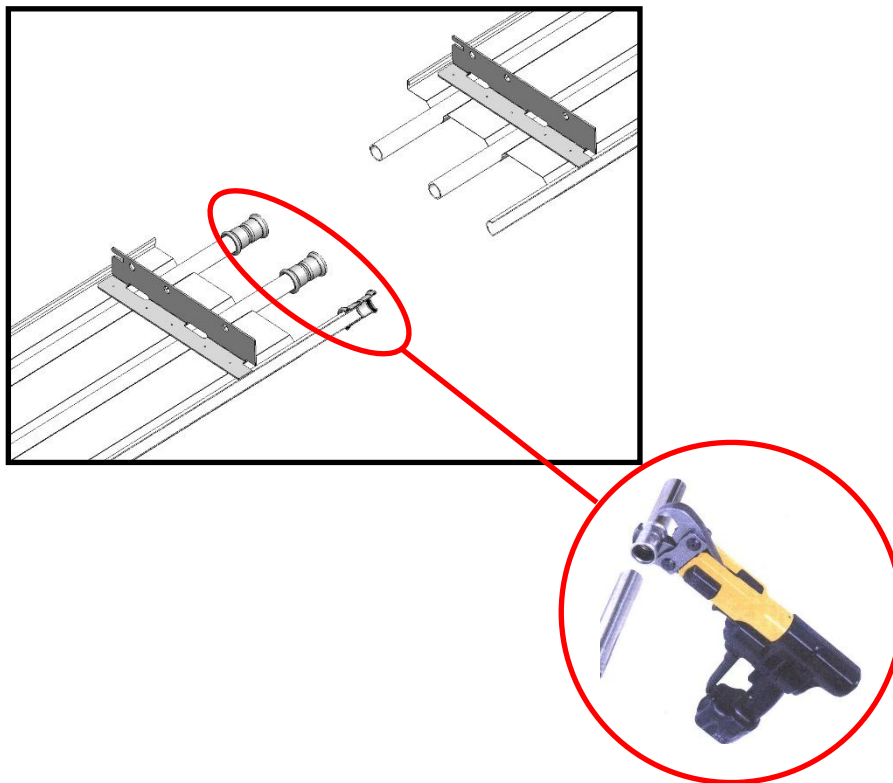
Fig. 3.13a Pinch the sleeve with the suitable tool
