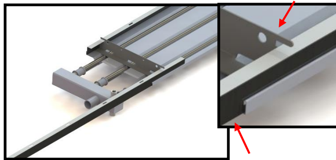
Fig. 3.17 Positioning of the side slats for the containment of the wool
