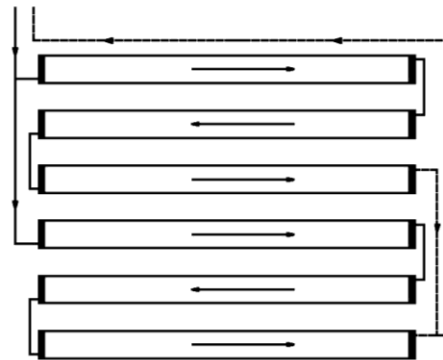
Inlet and outlet on opposite sides - 3 panels in sequence
