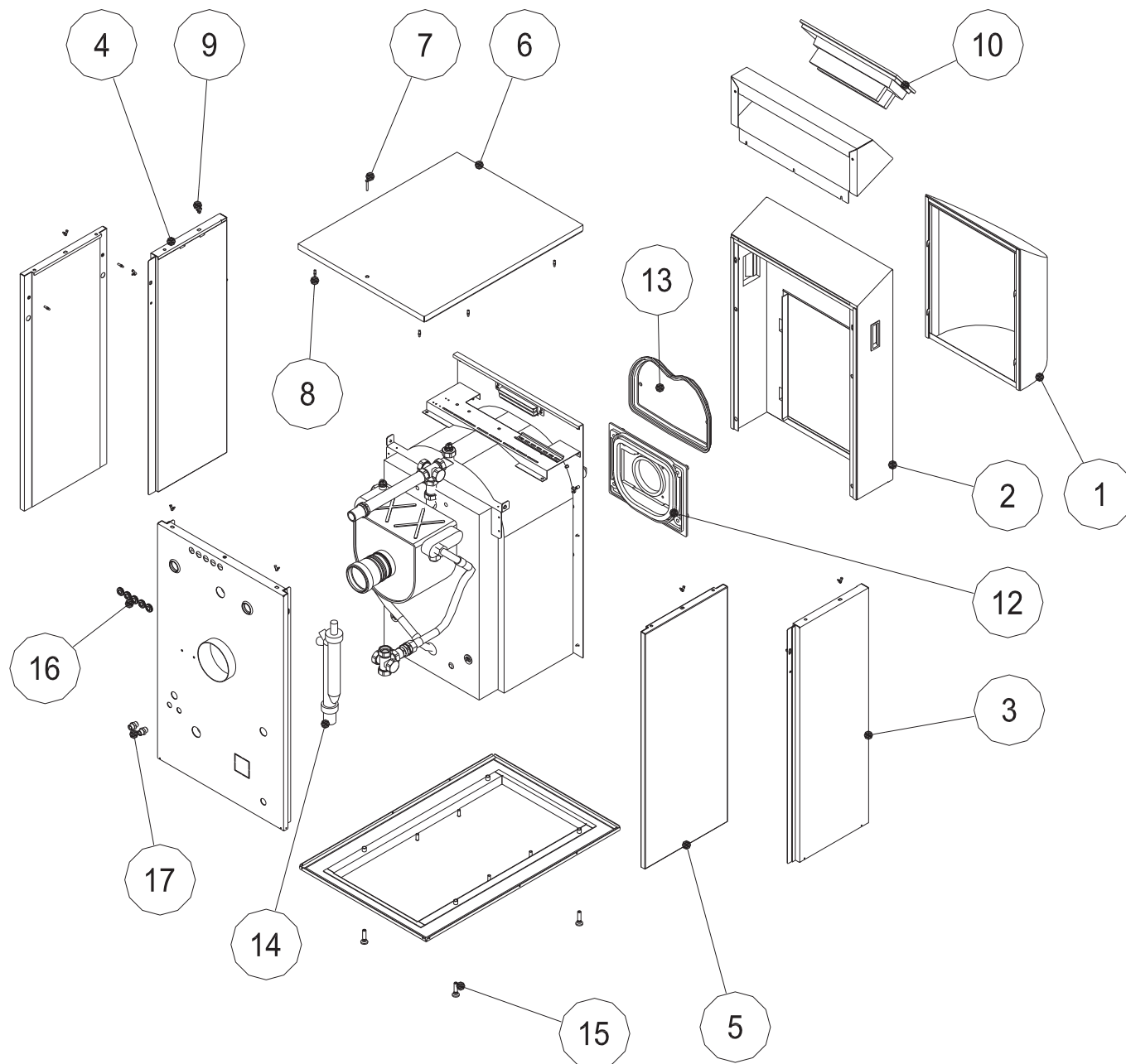
Fig. 51: Chaudière ecoOEL ...
